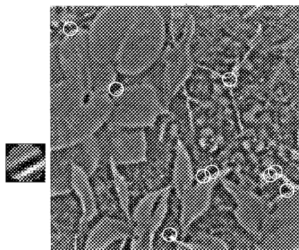
Figure 3: Patterns that yield high responses of a model neuron. The example receptive field is shown on the left. Some of the patterns that yield the strongest one-half percent of responses are labeled on the image on the right. These patterns are primarily the high-contrast edges.
