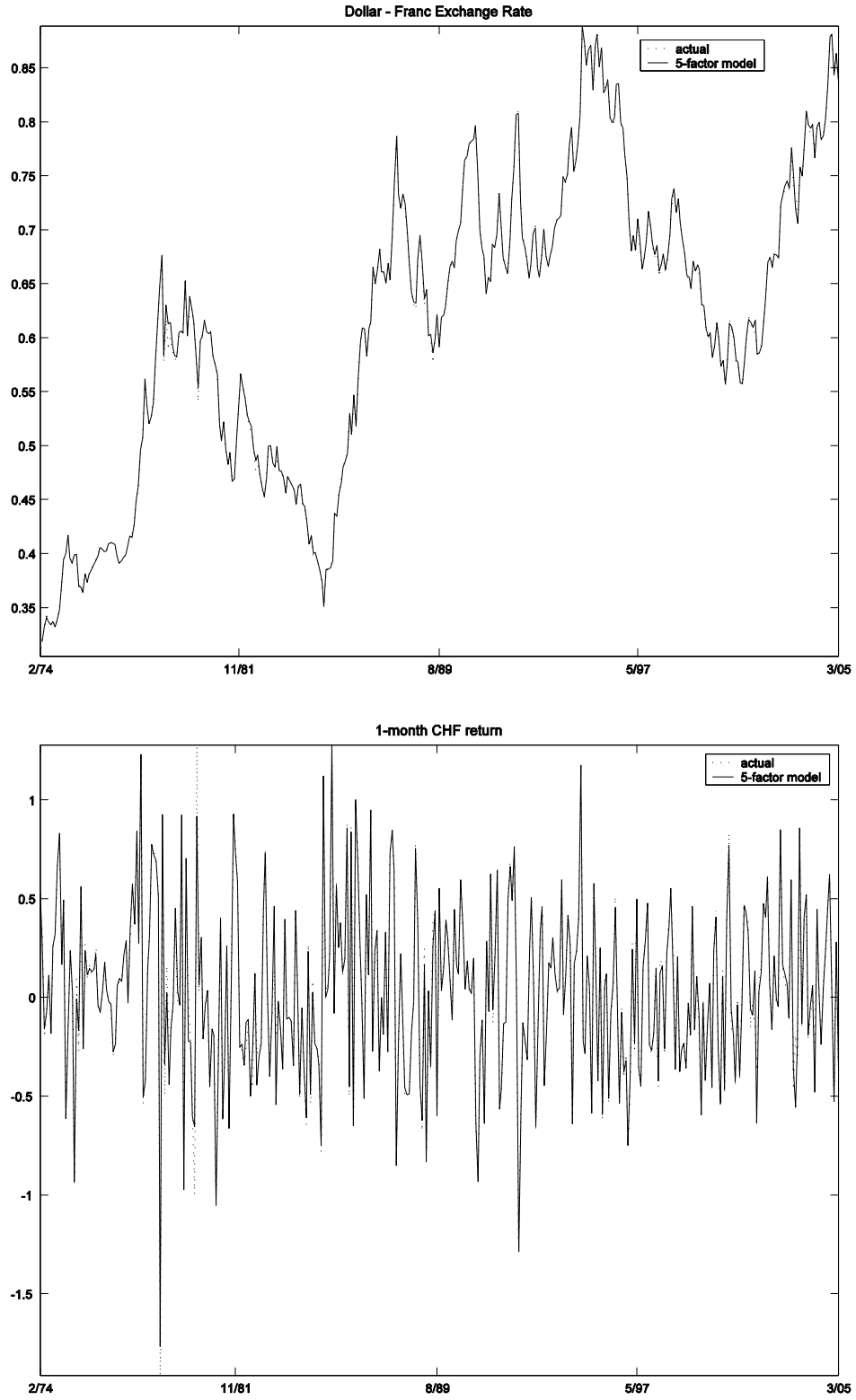
Fig. 7. Actual and five-factor model filtered US dollar-Swiss franc exchange rate and monthly return values.
